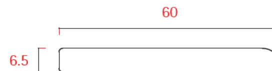
709038 - 60mm Architrave
