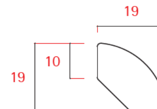
709041 - 19mm Quadrant
