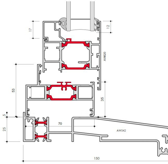
SQUARE (70MM)
