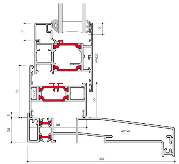
FLAT (58MM)
