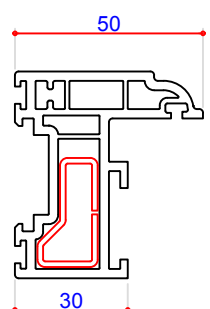
P10118 Upper Sash S000120 Steel Box
