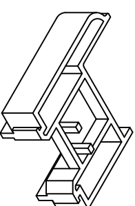
M00122 Vertical Slider End Cap (for mechanical joint fixing)
