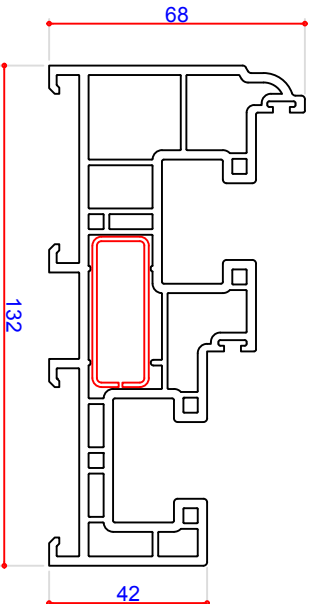
P101055 Cill S000016 Steel Box
