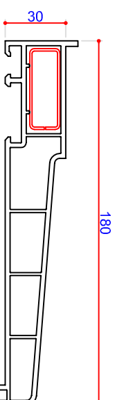
P90043 180mm Cill End Caps M00186 Steel 40 x 15 S00016 Straight Coupler M00188
