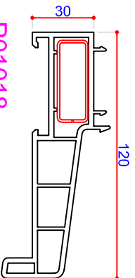
P01018 120mm Cill End Cap M00022 Steel 40 x 15 S00016
