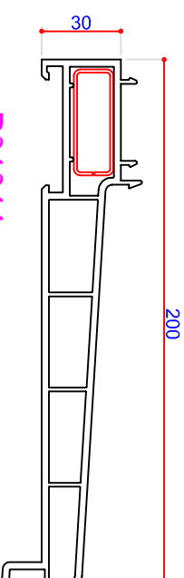
P01044 200mm Cill End Caps M00033 Steel 40 x 15 S00016
