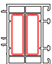
P01092 50mm Frame Ext Steel Box S000003
