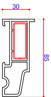
P90039 85mm Cill End Cap M00137 Steel 40 x 15 S00016
