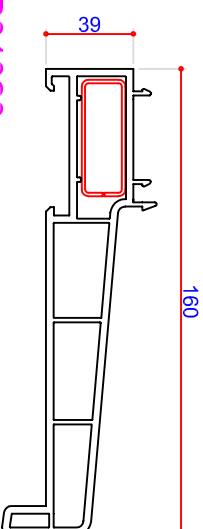
P01020 160mm Cill End Caps M00025 Steel 40 x 15 S00016 Straight Coupler M00116 90° Coupler M00196
