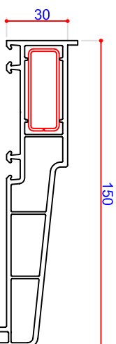
110103 150mm Cill End Caps 109006 Straight Coupler 109010 Steel 40 x 15 S00016
