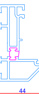
A00345 Aluminium Rebated Threshold
