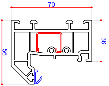
P10501 56mm Outer Frame Steel U Channel S00185 Thermal Insert P10331
