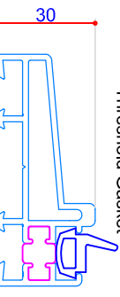
A00092 Standard Low Threshold
