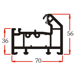
56mm OUTERFRAME P10501
