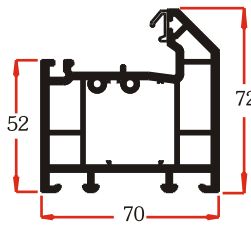
72mm OUTERFRAME P10502
