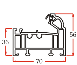
56mm OUTERFRAME P10531
