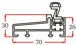
FLAT LOW THRESHOLD A00092 G52005 Threshold Seal
