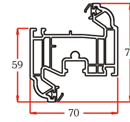
TILT AND TURN SASH P10539
