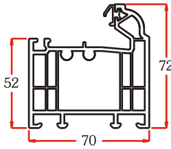
72mm OUTERFRAME P10532
